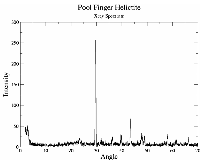
Figure 1 - Xray spectrum of Pool Finger helictite. Vertical scale: counts; horizontal scale: 2 \theta
