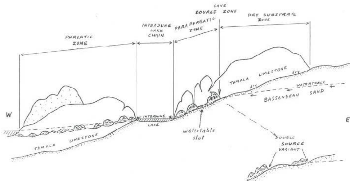
Figure 2 - Schematic east-west cross-section
