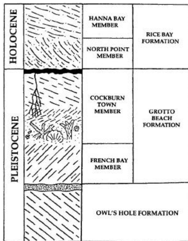
Figure 2 - Stratigraphic column for the Bahamas, illustrating the temporal relationships between units. Actual field relationships are rarely vertically stacked and are usually laterally adjacent (Carew and Mylroie 1995a)
