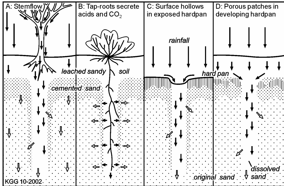
Figure 7 - Alternative ways to focus downward flow and generate solution pipes Note: the alternatives are not mutually exclusive, they could all contribute in different settings.
