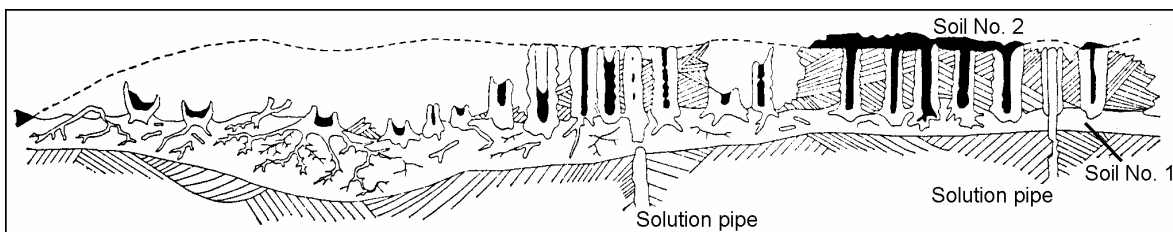
Figure 5 - Boutakoff's figure 17 shows many features of the "Petrified Forest" correctly but grossly exaggerates the thickness and extent of root development at the base of the pipes. Black is soil fillings.
