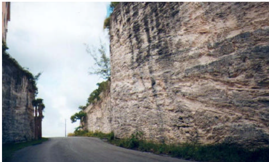
Figure 5 - Dune cross bedding, road cutting, New Providence Island
