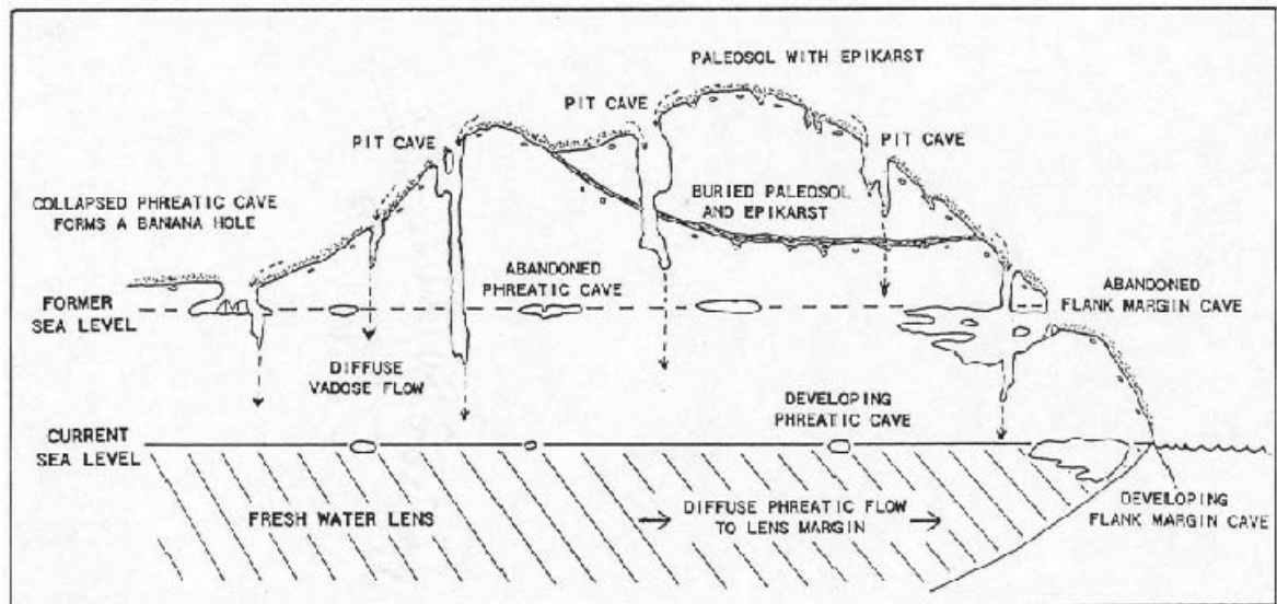
Figure 7 - Diagrammatic representation of the freshwater lens within a typical Bahamian island, showing the epikarst, pitcaves, banana holes and flank margin caves
