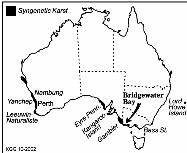
Figure 1 - Dune limestone areas in Australia
