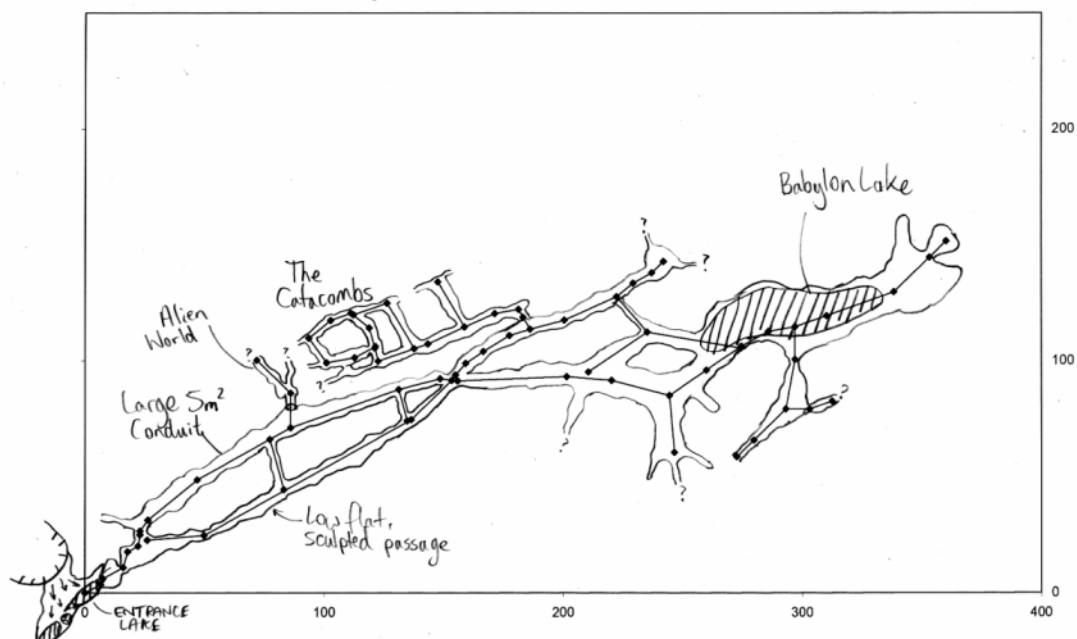
Figure 3 - Olwolgine Cave Sketch
